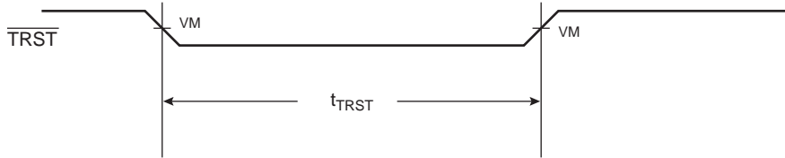
Figure 15. \overline{\text{TRST}} Timing Diagram
